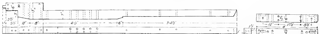
Figs. 1223-1224. Draw-timbers (4), 2 R & 2 L.
